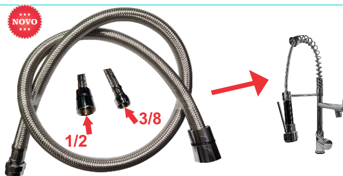
FLEX GOURMET IMPORTADO (55 CM P.SEXT 3/8 E P. CONICA 1/2)
